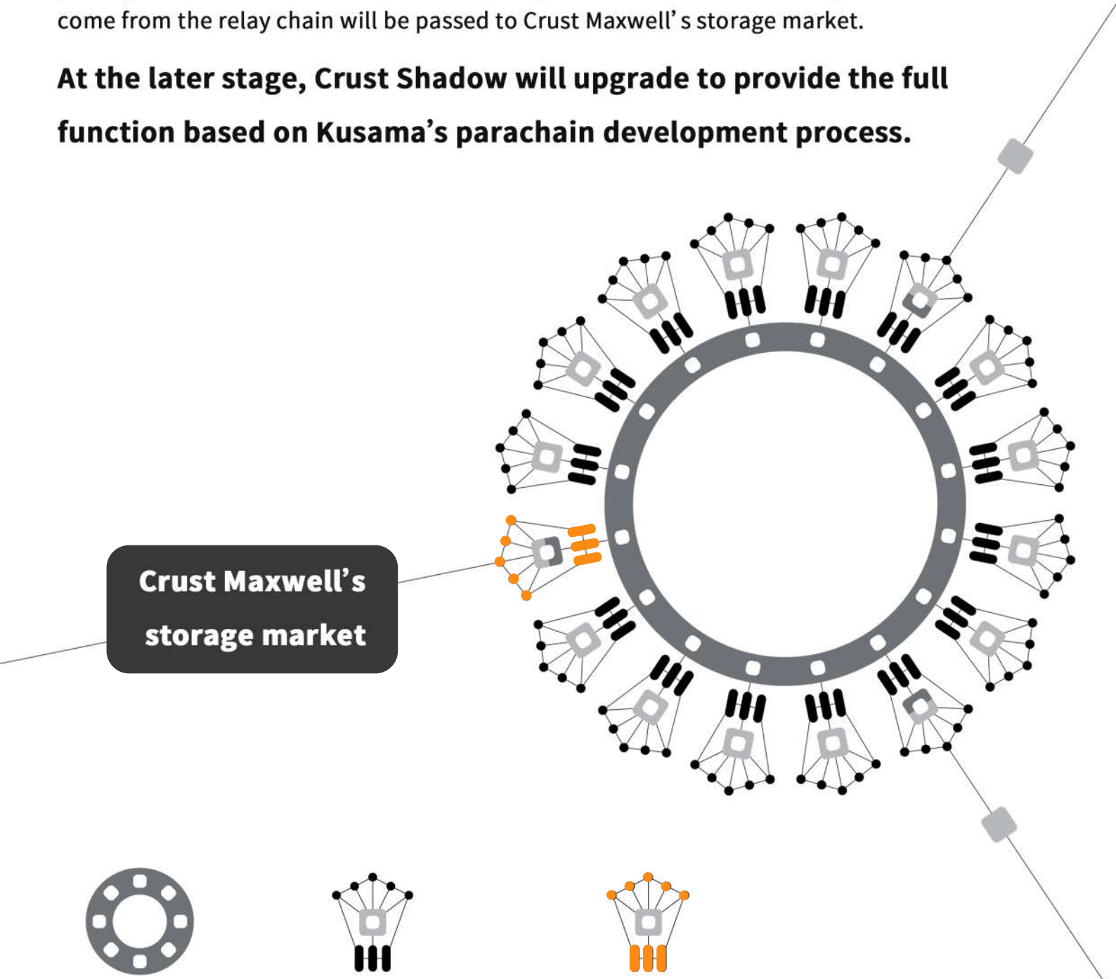
Relay Chain
